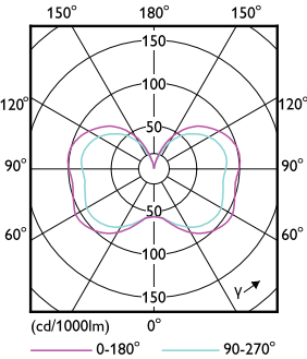
Light Distribution Diagram - 54-45-36CC/MAS/3PW/3CCT/Ex39 BB 3/1
