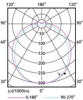
Light Distribution Diagram - CorePro LED PLT HF/Mains 6.5W 830 4P
