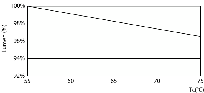
Lumen Maintenance Diagram - CorePro LED PLT HF/Mains 6.5W 830 4P
