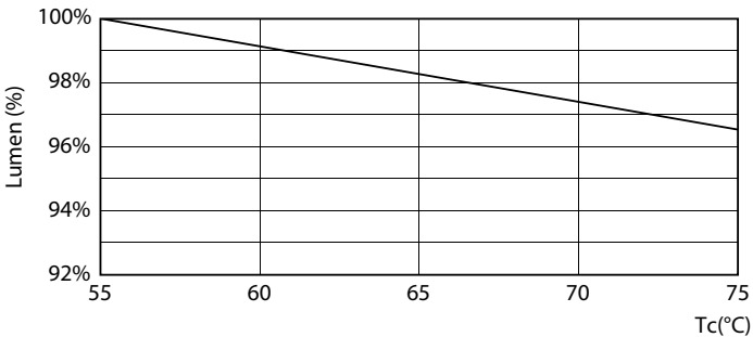
Lumen Maintenance Diagram - CorePro LED PLT HF/Mains 6.5W 840 4P
