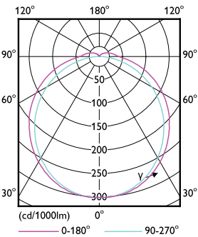
Light Distribution Diagram - CorePro LED PLT HF/Mains 6.5W 840 4P
