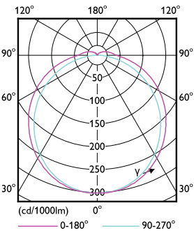
Light Distribution Diagram - CorePro LED PLT HF/Mains 9W 830 4P
