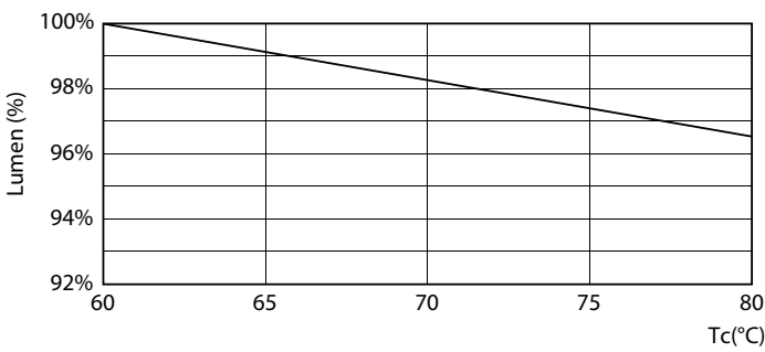
Lumen Maintenance Diagram - CorePro LED PLT HF/Mains 9W 830 4P
