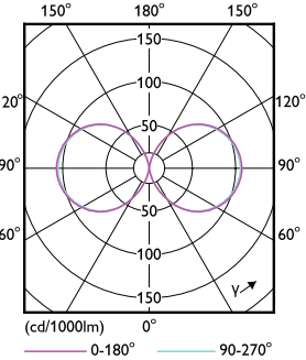
Light Distribution Diagram - 180-130-100CC/MAS/3PW/740/EX39 BB 3/1
