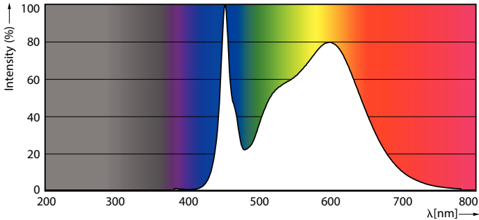
Spectral Power Distribution Colour - MAS LEDtube Mains/EL 1500mm 20W 840 T8
