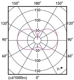
Light Distribution Diagram - CorePro LED HPL/SON M 4Klm 23W840E27 FR
