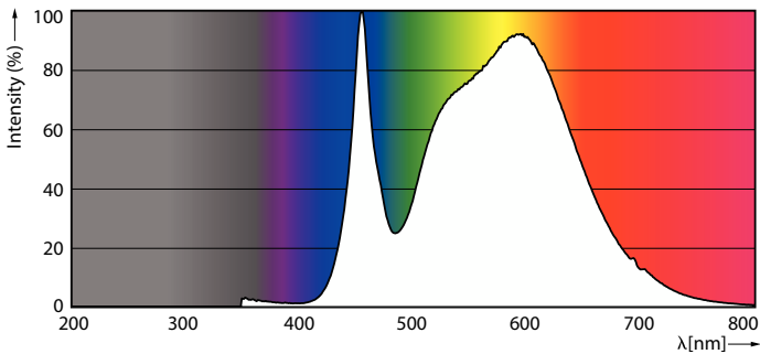
Spectral Power Distribution Colour - CorePro LED HPL/SON M 4Klm 23W840E27 FR
