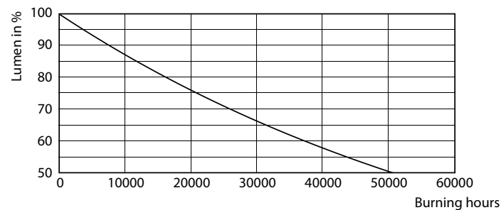
Lumen Maintenance Diagram - CorePro LED HPL/SON M5.3Klm28.5W827E27FR
