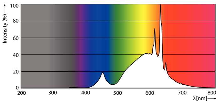
Spectral Power Distribution Colour - CorePro LED HPL/SON M5.3Klm28.5W827E27FR
