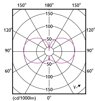
Light Distribution Diagram - CorePro LED HPL/SON M5.3Klm28.5W827E27FR
