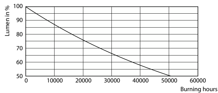
Lumen Maintenance Diagram - CorePro LED HPL/SON M5.5Klm29.5W830E27FR
