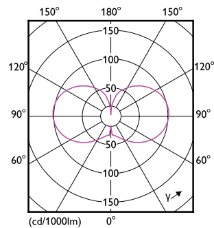
Light Distribution Diagram - CorePro LED HPL/SON M5.5Klm29.5W830E27FR
