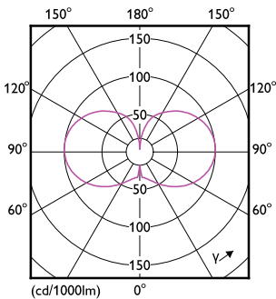
Light Distribution Diagram - CorePro LED HPL/SON M5.5Klm29.5W830E40FR
