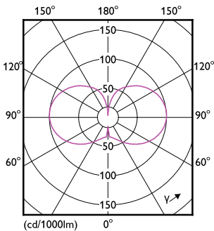
Light Distribution Diagram - CorePro LED HPL/SON M 6Klm 31W 840 E40FR
