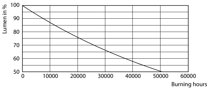
Lumen Maintenance Diagram - CorePro LED HPL/SON M 6Klm 31W 840 E40FR
