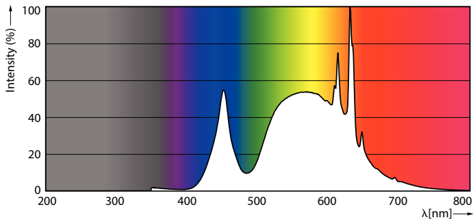
Spectral Power Distribution Colour - CorePro LED HPL/SON M 6Klm 31W 840 E40FR
