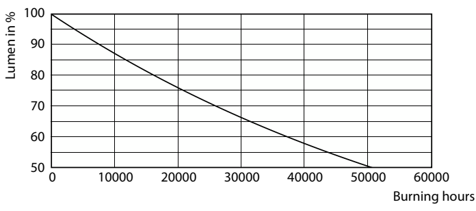
Lumen Maintenance Diagram - CorePro LED HPL/SON M 6Klm 31W 840 E40FR
