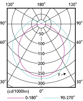
Light Distribution Diagram - 6PL-S/COR/13H-5CCT/MF6/P/2P 20/1
