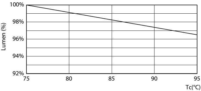
Lumen Maintenance Diagram - 8PL-L/COR/18-5CCT/MF9/G/4P 10/1
