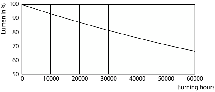
Lumen Maintenance Diagram - 8PL-L/COR/18-5CCT/MF9/G/4P 10/1
