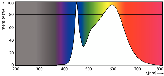
Spectral Power Distribution Colour - 8PL-L/COR/18-5CCT/MF9/G/4P 10/1
