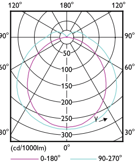
Light Distribution Diagram - 8PL-L/COR/18-5CCT/MF9/G/4P 10/1
