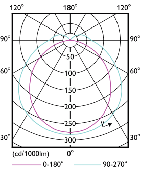
Light Distribution Diagram - 18PL-L/COR/55-5CCT/MF28/G/4P 10/1
