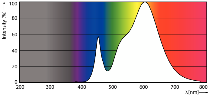
Spectral Power Distribution Colour - Corepro LEDBulbND 3.2Klm 30W830 E27T100
