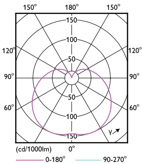
General uniform lighting - Corepro LEDBulbND 3.2Klm 30W830 E27T100
