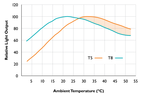
Relative Light Output vs. Ambient Temperature
