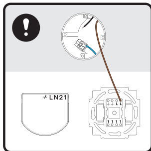
6. Replace with a new single push switch. Connect the line wire to the switch.
