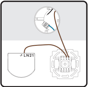
7. Place a new line wire between L terminal and the switch.
