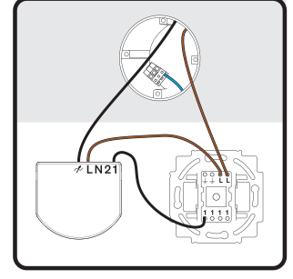
9. Place the load wire from the wall in the LN21 terminal
