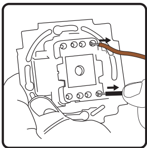
5. Remove the original dimmer completely
