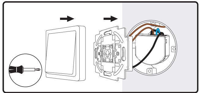
12. Remount the switch
