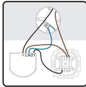
8. Place a new load wire between 1 terminal and the switch
