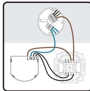
10. Place a new load wire between 1 terminal and the switch
