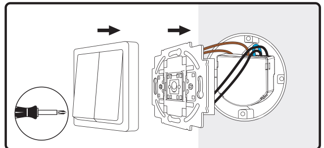
13. Remount the switch
