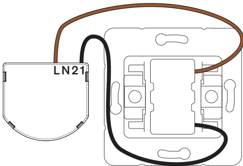
Standard switch with side mounting
