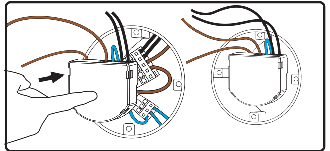
12. Fit the Hue module inside the wall box behind your existing switch
