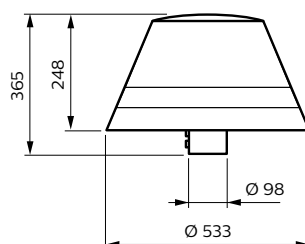
BDP262-62 of 76 + ring
