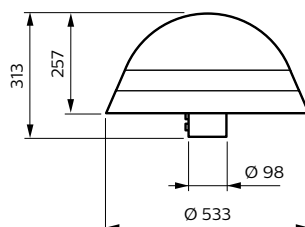
BDP263-62 of 76 + ring
