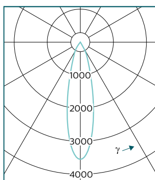
CustomCreate PT520T LED65S/830 MB Faisceau semi-extensif
