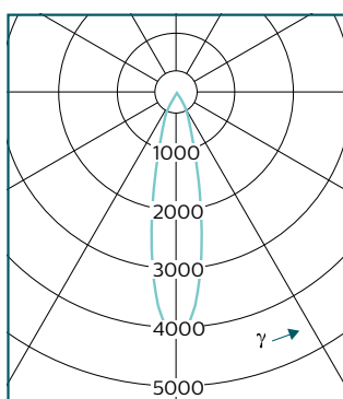
CustomCreate PT520T LED27S/830 MB Faisceau semi-extensif
