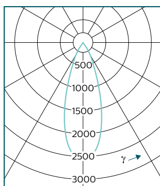
CustomCreate PT520T LED27S/830 WB Faisceau extensif
