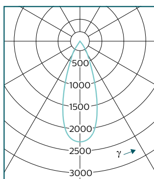
CustomCreate PT520T LED65S/830 WB Faisceau extensif
