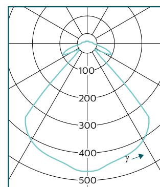
CustomCreate PT520T LED80S/830 DF Faisceau lambertien
