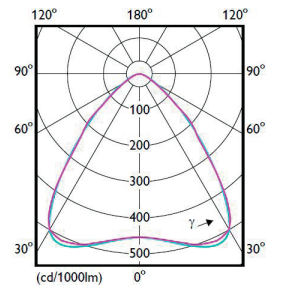
(cd/1000lm) 0° 90-270° SM340C, PCS, BAP-tauglich
