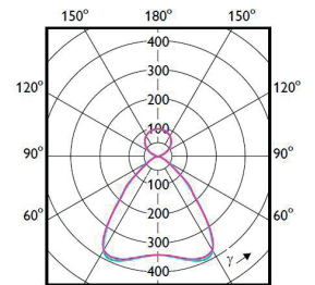
(cd/1000lm) 0-180° 90-270° SP342P, PCS, BAP-tauglich
