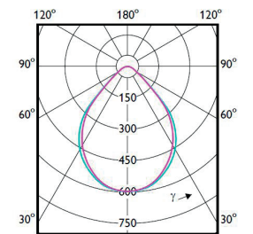
(cd/1000lm) 0° 90-270° Optional: SM340C, MLO, BAP-tauglich
