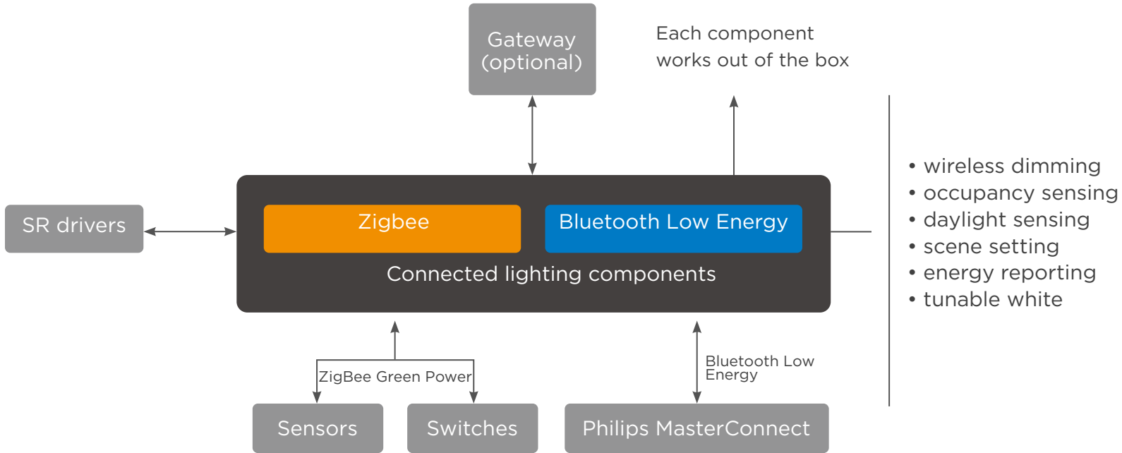
Figure 9: The Philips field app MC enables connected lighting networks based on open standards.
