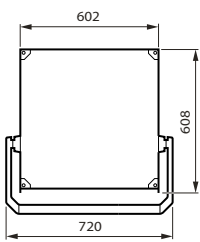
ClearFlood Large BVP 657 - Dimensions en mm
