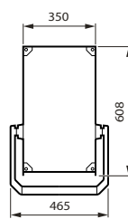
ClearFlood Medium BVP656 - Dimensions en mm
