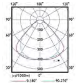
SM402C, Langfeld
