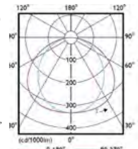
RC132V G4/RC133V G4 NOC
