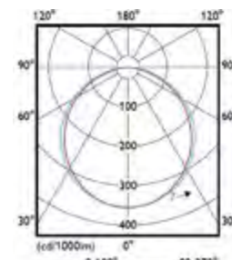
SM531C, opal
