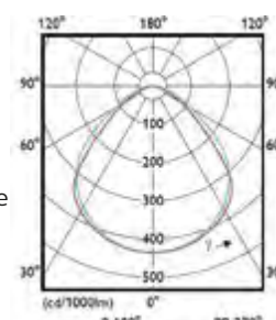
SM136V NOC
