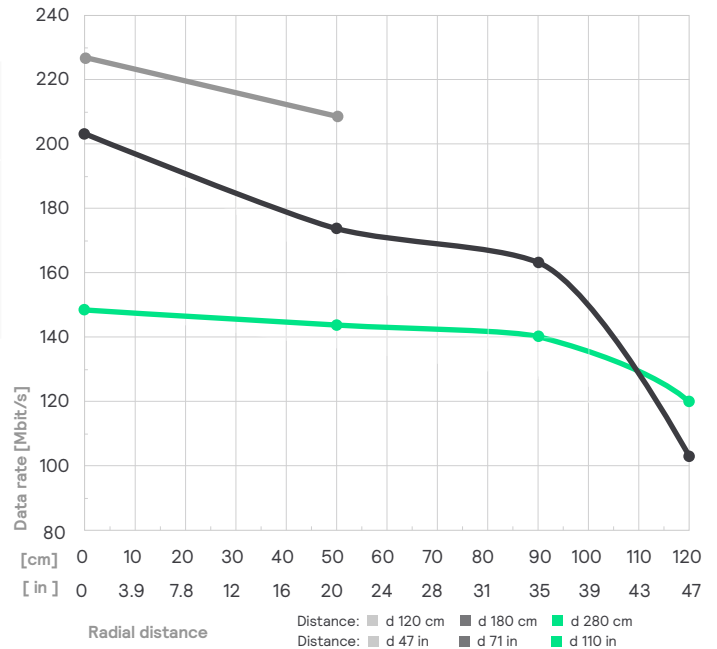
Figure 2: Downlink data rate
