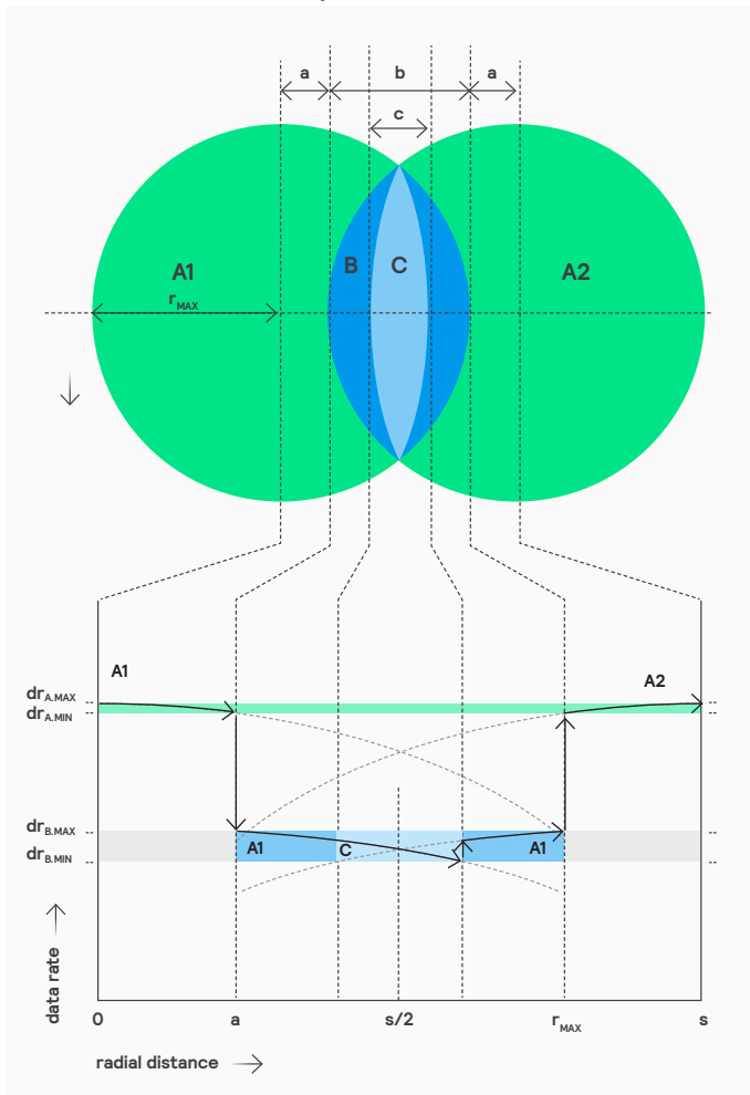
Figure 6: Handover scenario between overlapping coverage areas
