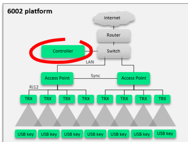
Example set-up of 6002 based system.
