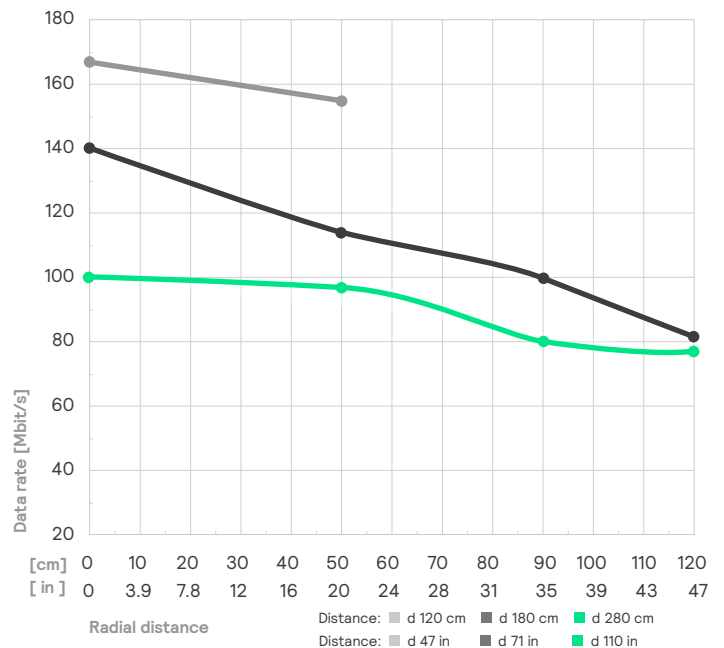
Figure 3: Uplink data rate
