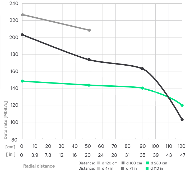
Figure 2: Downlink data rate
