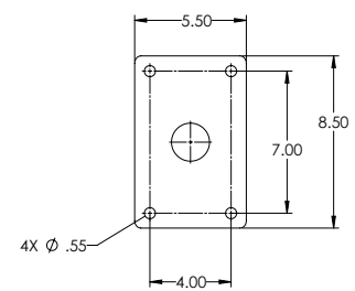
Mount plate
