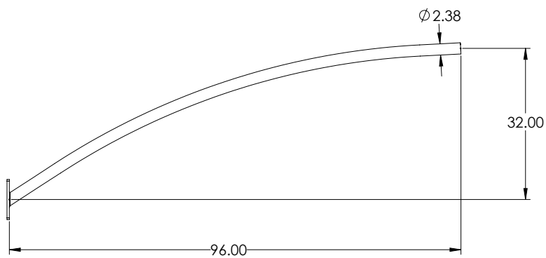
8ft Arm
