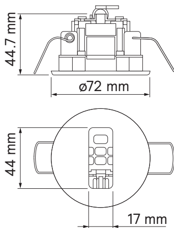
recessed holder
