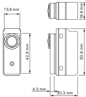
sensor SC200
