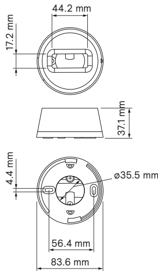
surface mounted holder
