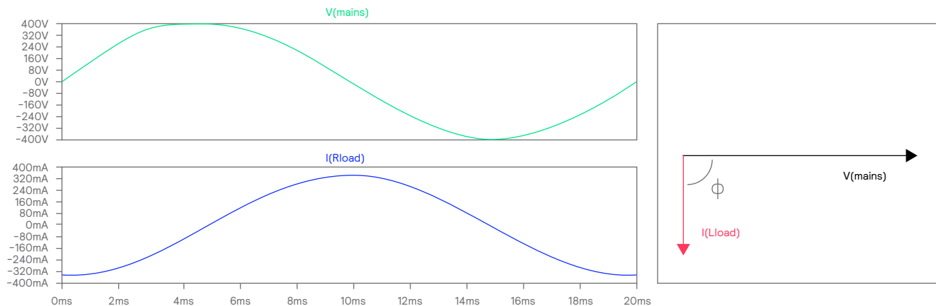
Figure 2: Voltage and current waveform of inductive load (green = voltage, blue = current)
