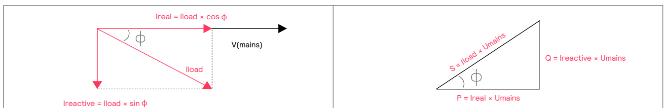
Figure 5: A: current decomposition, B: power triangle
