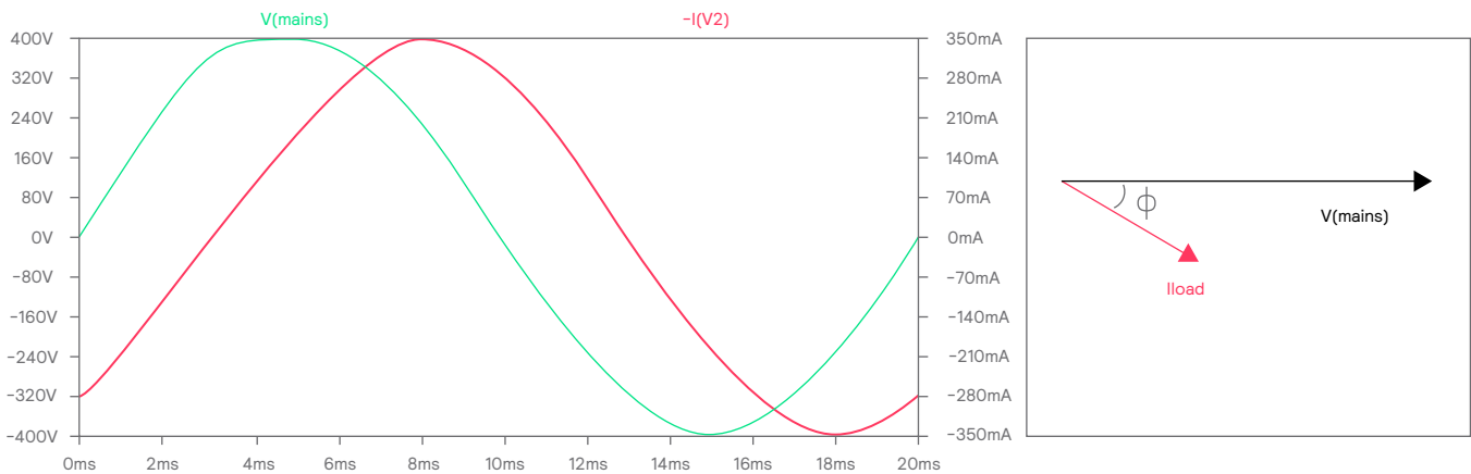
Figure 4: Voltage and current waveform of conventional lighting load (green = voltage, red = current)
