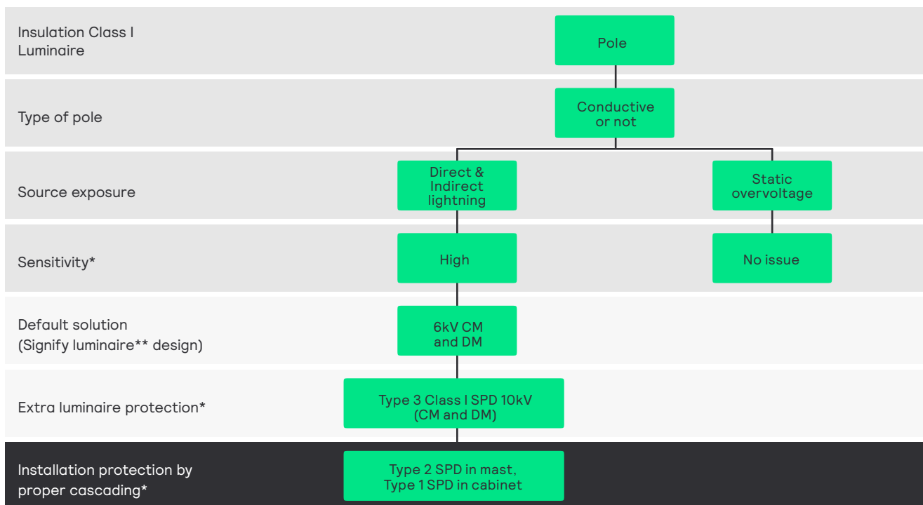
Figure 7: Surge protection class I: Installation level
