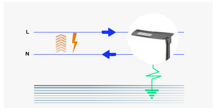
Figure 2: Definition of differential mode current flow
