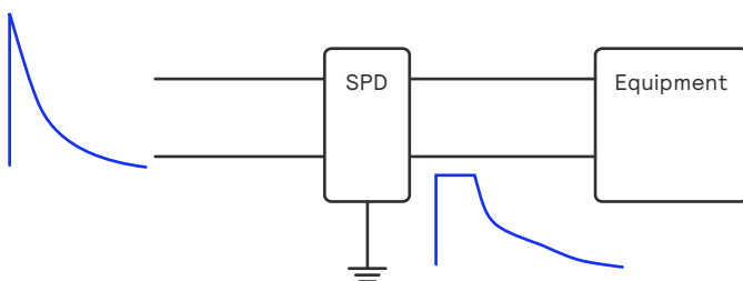
Figure 4: Working principle of a surge protection device (SPD)
