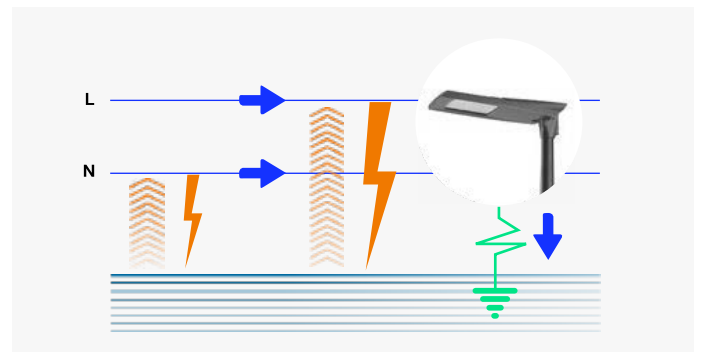
Figure 3: Definition of common mode current flow
