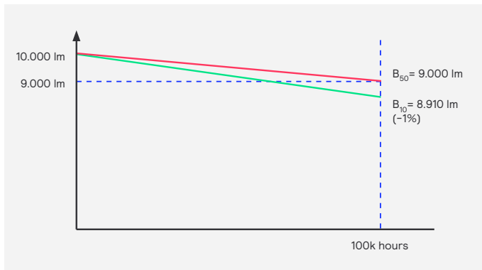
Figure 1: Product data analysis of an example of a LED based luminaire
