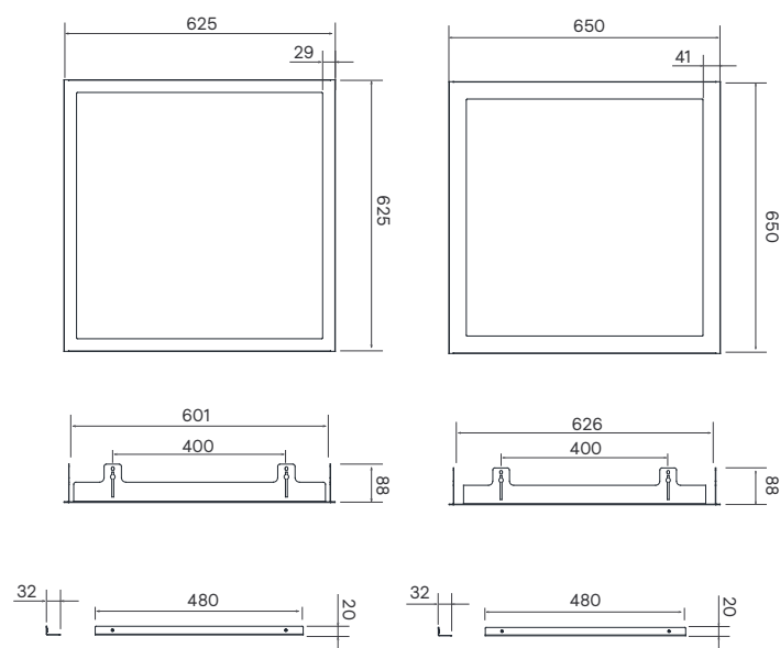
LP913Z NC3 PLASTER CEILING SET W60L60
