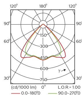
WB-OC (Wide beam – Office compliant)
