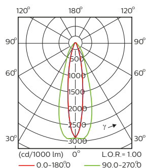
XNB (Extra narrow beam)
