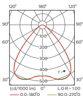
WB (Wide beam)
