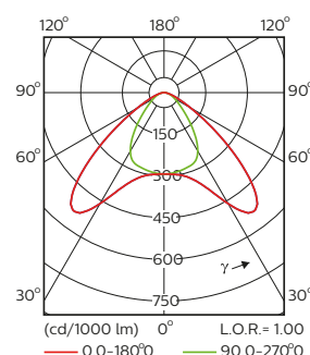
DA35W (Double asymmetric Wide)
