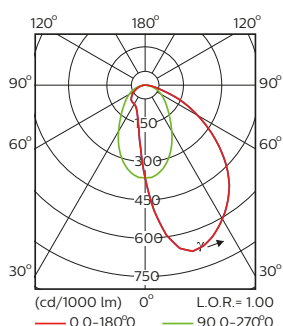
A20 (Asymmetric beam)
