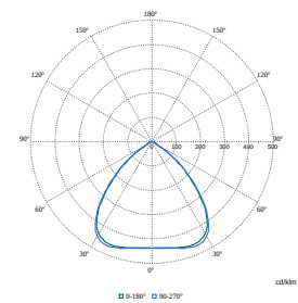
Polar Normal (separate) - BY580PI - 910505104554
