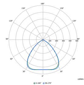
Polar Normal (separate) - BY580PI - 910505104556
