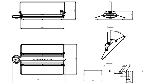
BY581X Bracket
