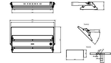
BY581X Bracket
