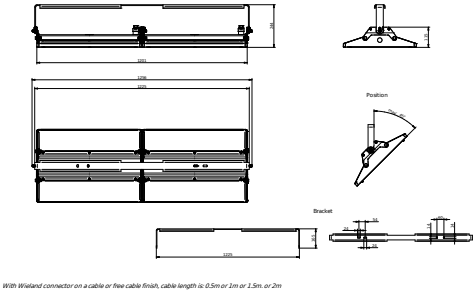
700S Bracket
