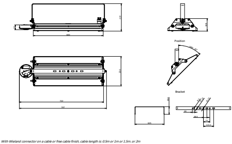
BY580X Bracket
