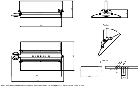
BY581X Bracket
