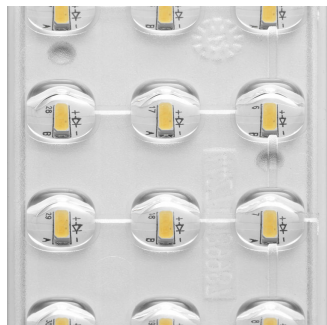
IPDP_4MX400i_0003-Detail photo
