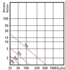
Accent Diagram - MAS LED ExpertColor 6.7-35W MR16 927 60D
