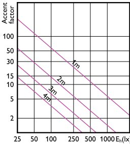
Accent Diagram - LED 14-120W PAR38 827 25D
