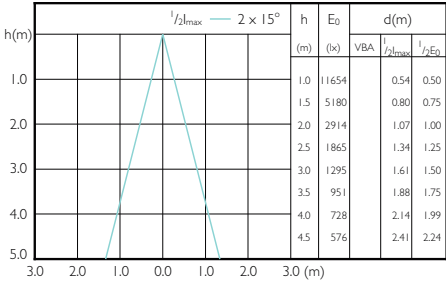
Beam diagram - Master LED PAR30L 32W 30D 830 220V
