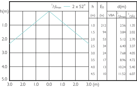
Beam diagram - 13.5PAR38/PER/ GREEN/G/E26/ND/ULW 3/1PF
