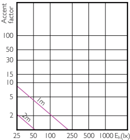
Accent Diagram - 13.5PAR38/PER/ GREEN/G/E26/ND/ULW 3/1PF
