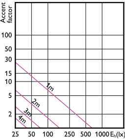
Accent Diagram - 4GU10/LED/930/F35/DIM/G/ 120V T20 10/1
