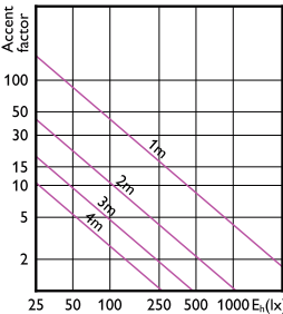
Accent Diagram - 10PAR38/COR/930/F25/DIM/P/ULW/T20 6/1FB
