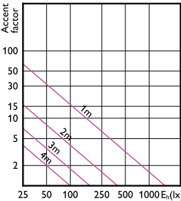
Accent Diagram - 6PAR38/90W/UE/ 930/40D/D/G/ULW/E26/T20/2P
