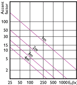
Accent Diagram - 13PAR38/COR/950/F25/DIM/P/ULW/T20 6/1FB
