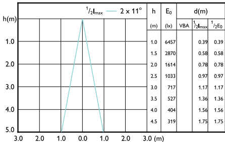
Beam diagram - PAR38 13-120W 930 25D G ULW Dim E27
