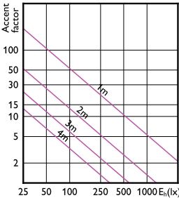
Accent Diagram - 13PAR38/COR/950/F40/DIM/P/ULW/T20 6/1FB
