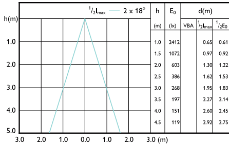
Beam diagram - MAS LEDEExpertColor 20-100W 927 AR111 24D
