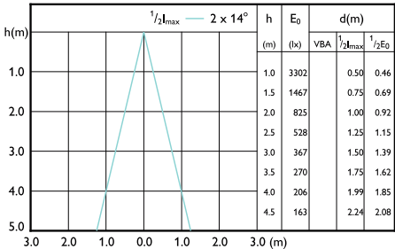
Beam diagram - MAS LEDExpertColor 20-100W 940 AR111 24D
