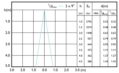
Beam diagram - MAS LEDEExpertColor 20-100W 930 AR111 15D
