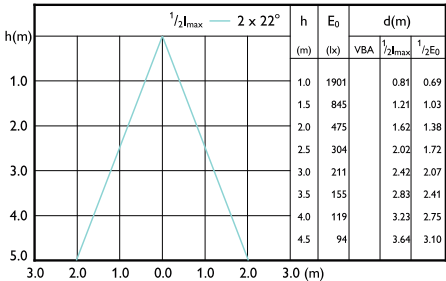
Beam diagram - MAS LEDExpertColor 20-100W 930 AR111 45D
