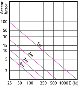
Accent Diagram - MAS LEDExpertColor 20-100W 930 AR111 24D
