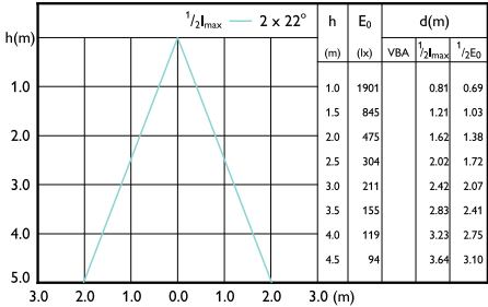
Beam diagram - MAS LEExpertColor 20-100W 930 AR111 45D
