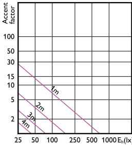
Accent Diagram - MAS ExpertColor 10.8-50W 930 AR111 24D
