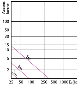
Accent Diagram - MAS ExpertColor 14.8-75W 927 AR111 45D
