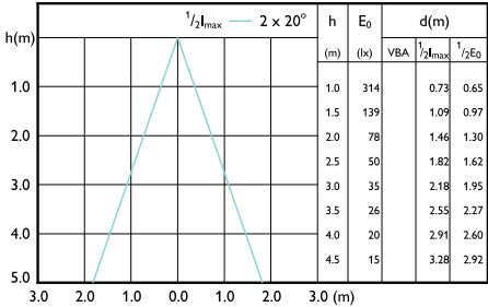
Beam diagram - MAS ExpertColor 10.8-50W 927 AR111 40D
