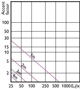
Accent Diagram - MAS ExpertColor 10.8-50W 927 AR111 24D
