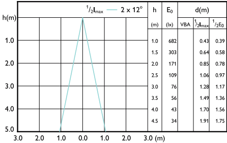
Beam diagram - MAS ExpertColor 10.8-50W 930 AR111 24D
