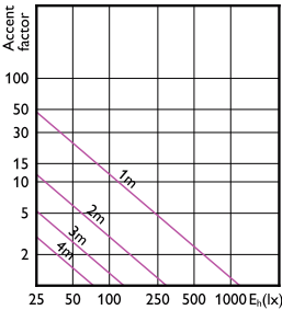
Accent Diagram - CorePro LEDspot 7-50W 830 AR111 40D
